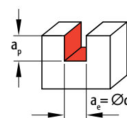
Slot milling
